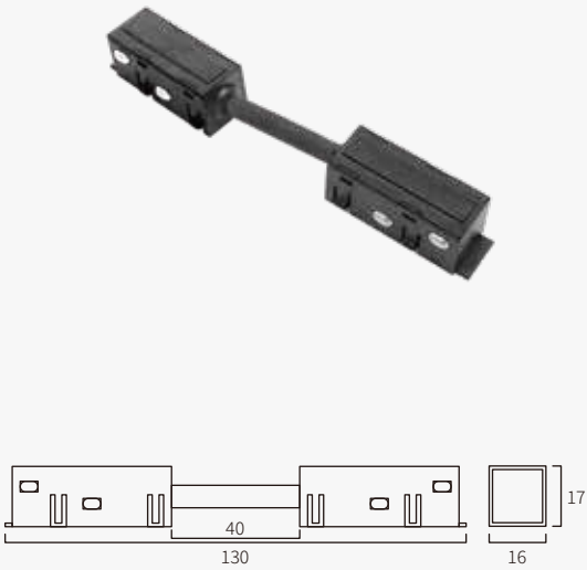
I connector
