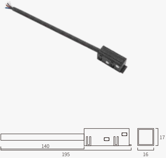
Feeder
